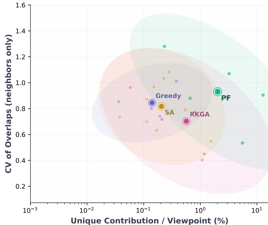
CV of Overlap vs Viewpoint Unique Contribution
